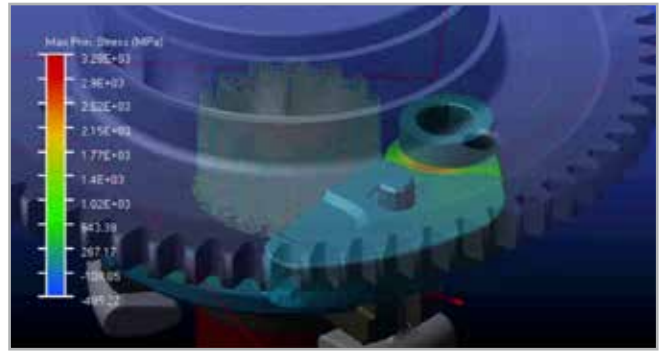
Fig. 13 - The rotating bodies' structural performance and the modal superposition results.
