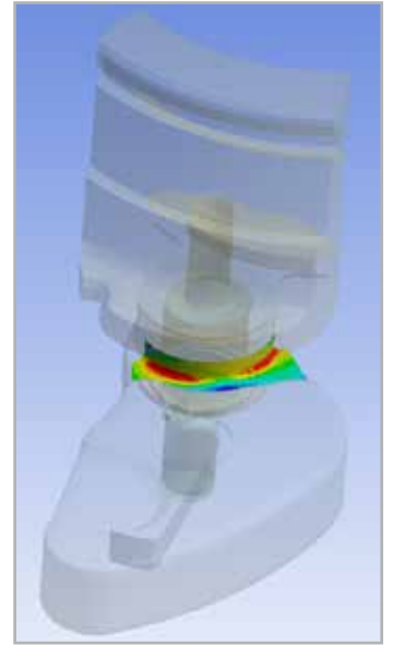
Fig. 14 - The rotating bodies' structural performance and the stress distribution computed with an explicit FEM model.
