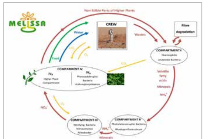
Fig. 1 - The MELiSSA Loop
