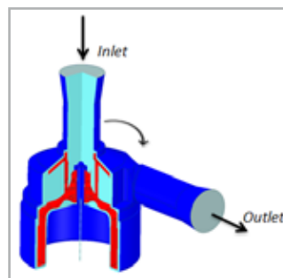
Fig. 4 - Computational domain of the fluid-dynamics simulation.
