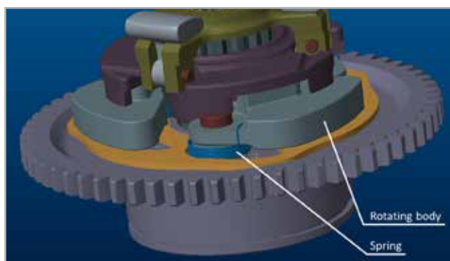
Fig. 2 - Rotating bodies.
